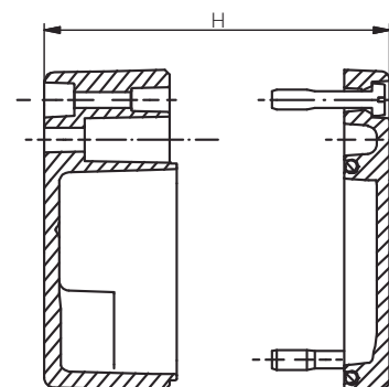
Schnitt A - A cutaway model A - A
