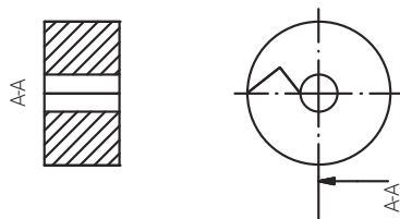
Dichtring Sealing
